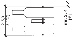
Regular - 1 Bottle (P1) - 2 SIDES
