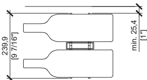
Magnum - 1 Bottle (MP1) - 2 SIDES
